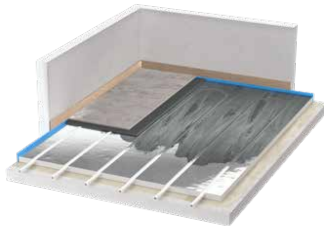
Kilma Futura system with ceramic covering glued directly onto the panel
